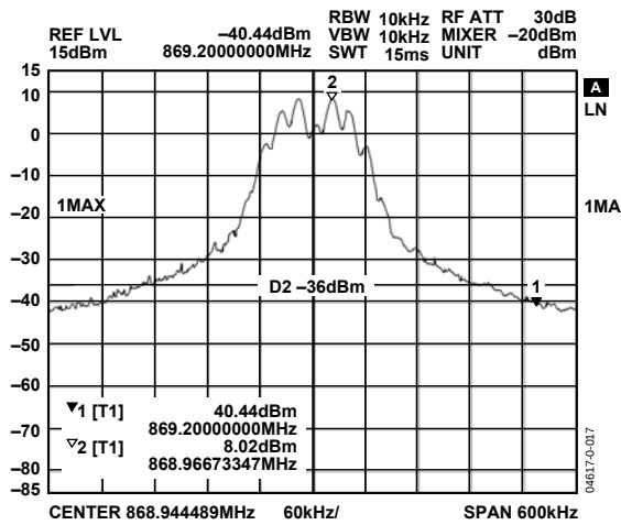
Figure 17. FSK Modulation, Power = 12.5 dBm, Data Rate = 38.4 kbps, F_{\text{DEVIATION}} = \pm 19.2 \text{ kHz}
