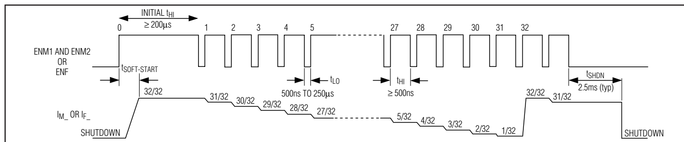
Figure 1. ENM_ and ENF Timing Diagram
