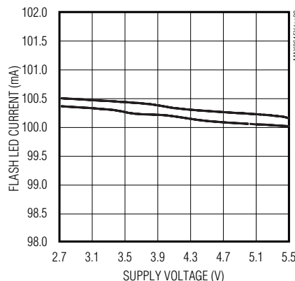
LED CURRENT MATCHING vs. SUPPLY VOLTAGE WITH TWO FLASH LEDs
