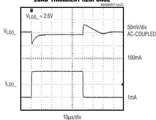
LOAD-TRANSIENT RESPONSE
