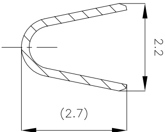
SECT "B"-"B"
