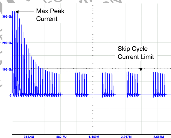
Figure 19. The skip cycle takes place at low peak currents which guarantees noise free operation
