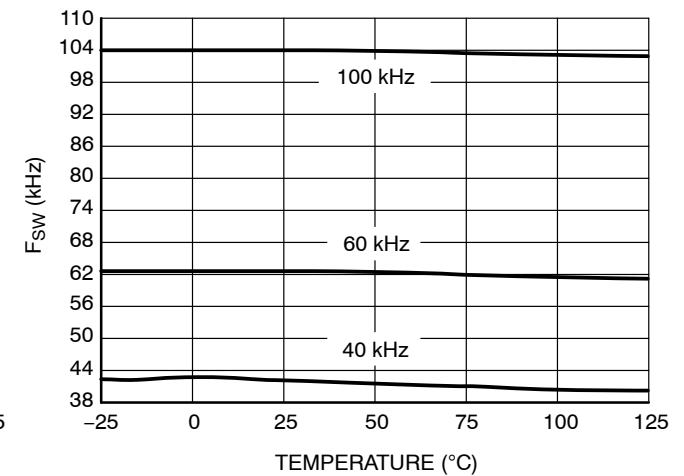
Figure 8. Switching Frequency vs. T j
