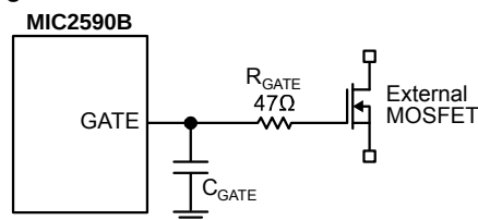
Figure 12. Proper Connection of C GATE and R GATE
