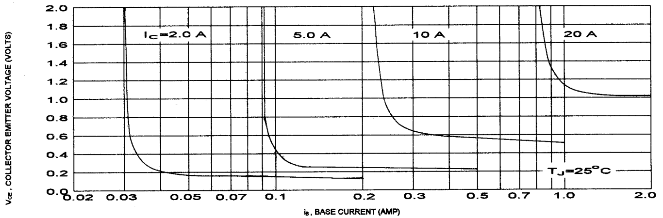
"ON" VOLTAGES
