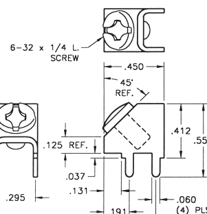
PC MOUNT
