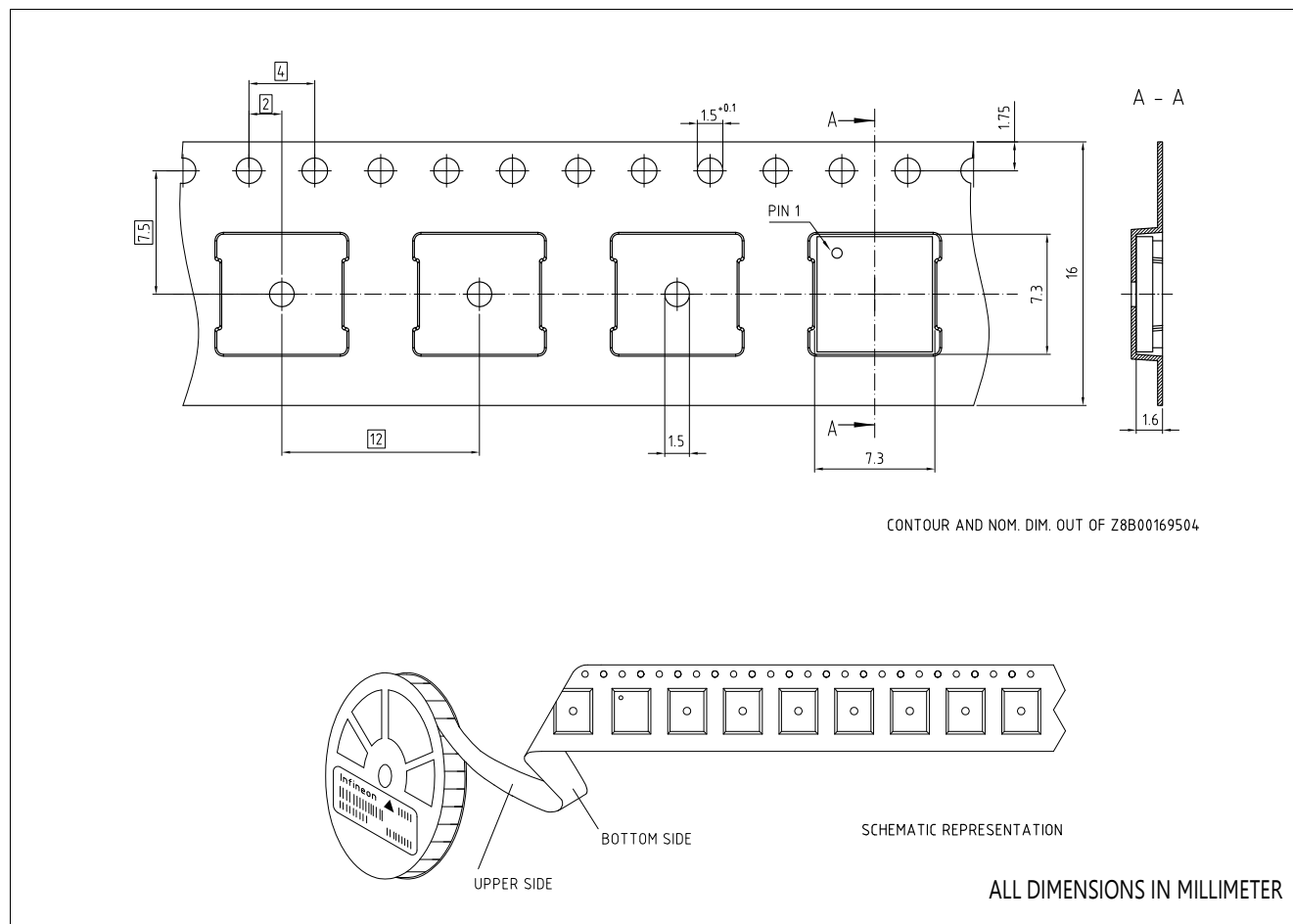
Figure 5-2 Carrier tape of the PG-TISON-8-1 package
