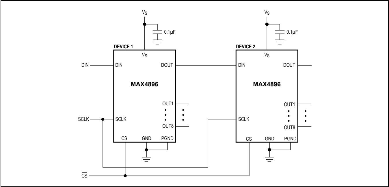
Figure 3. Daisy-Chain Configuration
