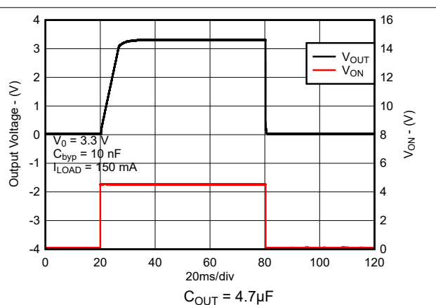
Figure 7-29. Turn-On Time (New Chip)
