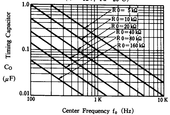
VCO Frequency
