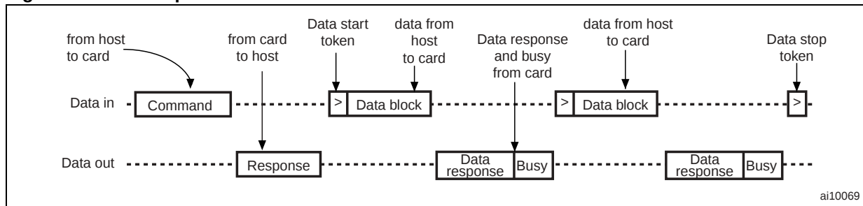
Figure 36. Write operation
