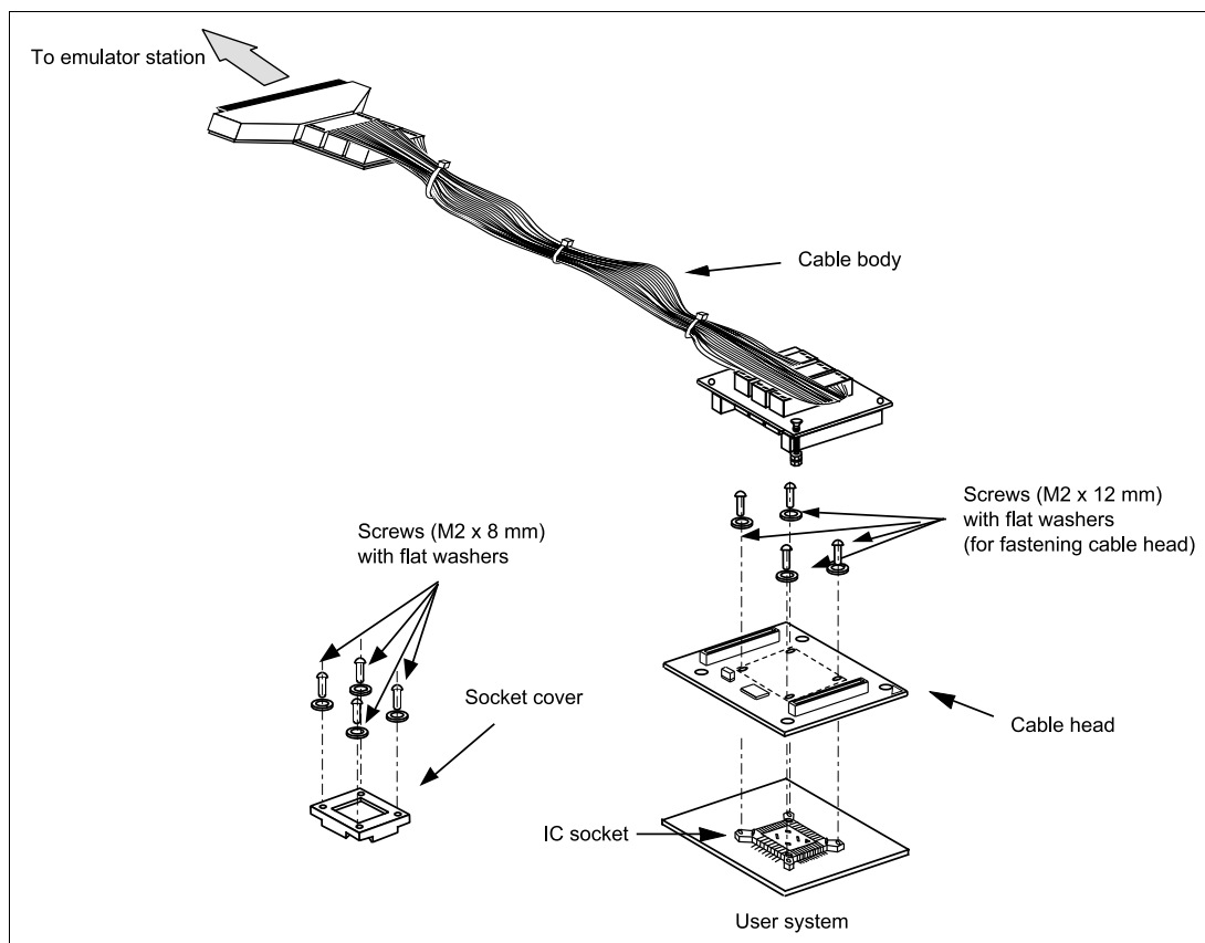
Figure 1 HS3644ECH61H User System Interface Cable
