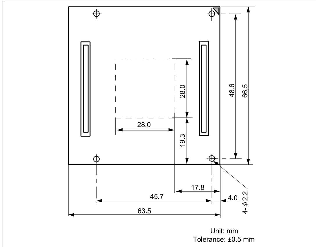
Figure 6 Dimensions for User System Interface Cable Head
