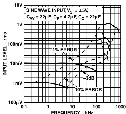
TPC 4. Frequency Response Driving Pin 1
