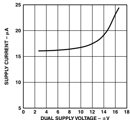
TPC 3. Power-Down Current vs. Supply Voltage
