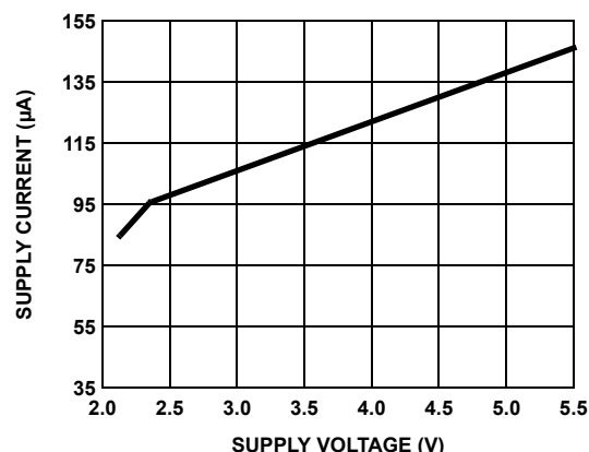
FIGURE 15. ISL28286 SUPPLY CURRENT vs SUPPLY VOLTAGE
