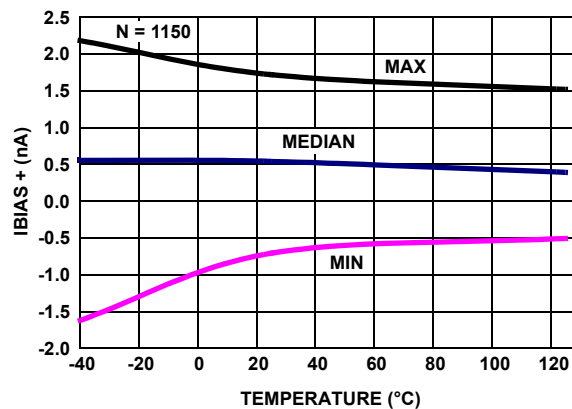
FIGURE 20. I_{BIAS +} vs TEMPERATURE, V_+ , V_- = \pm 2.5V
