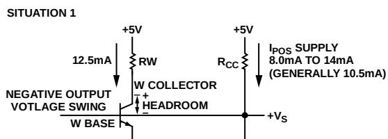
Figure 14. Negative Swing
