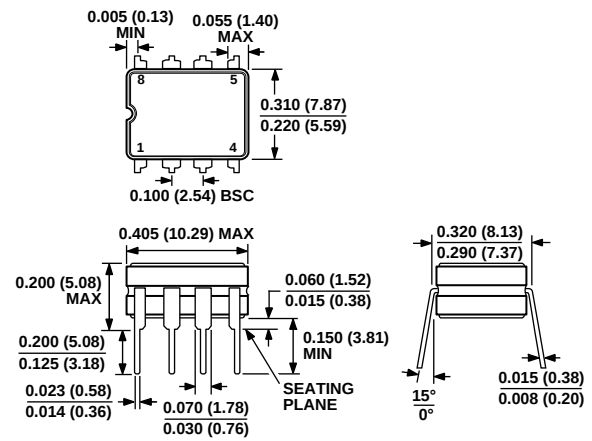
Figure 25. 8-Lead Ceramic Dual In-Line Package [CERDIP] (Q-8)
