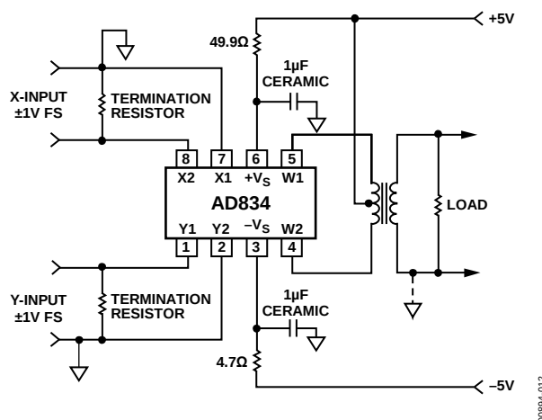
Figure 16. Transformer-Coupled Output
