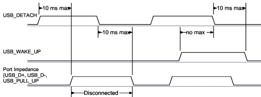
USB_DETACH and USB_WAKE_UP Signal
