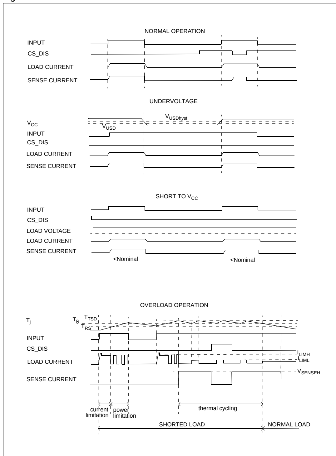
Figure 10. Waveforms
