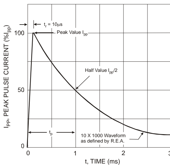
Fig. 2 Pulse Waveform
