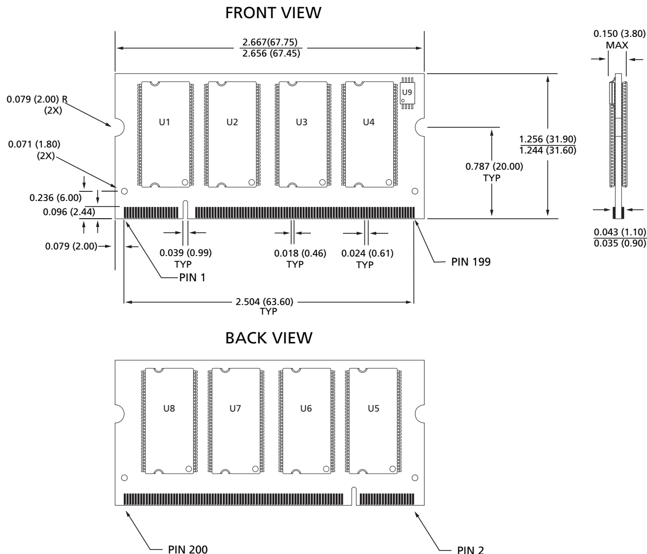
Figure 15: 200-Pin DDR SODIMM Dimensions
