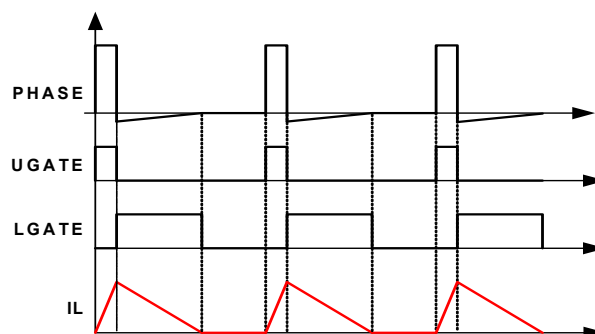
FIGURE 6. DIODE EMULATION
