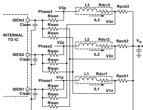
FIGURE 11. DIFFERENTIAL-SENSING CURRENT BALANCING CIRCUIT
