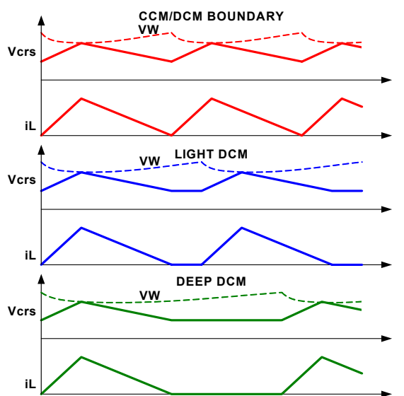
FIGURE 7. PERIOD STRETCHING
