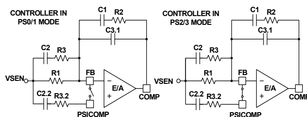
FIGURE 15. PSICOMP FUNCTION
