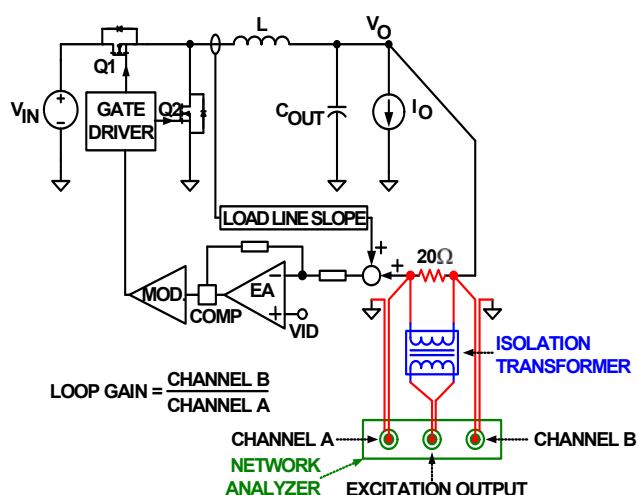
FIGURE 25. LOOP GAIN T2(s) MEASUREMENT SET-UP
