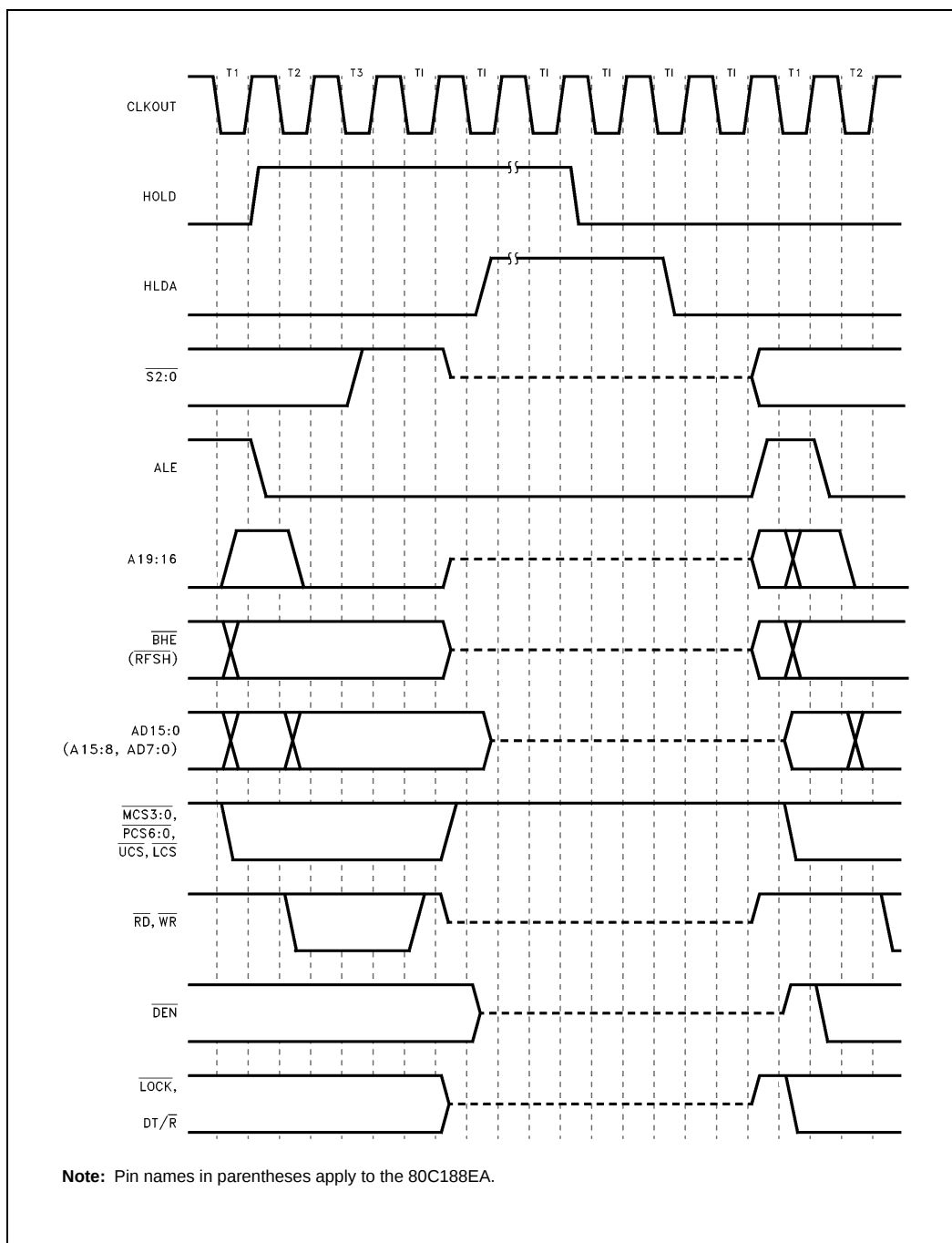
Figure 17. HOLD/HLDA Waveform
