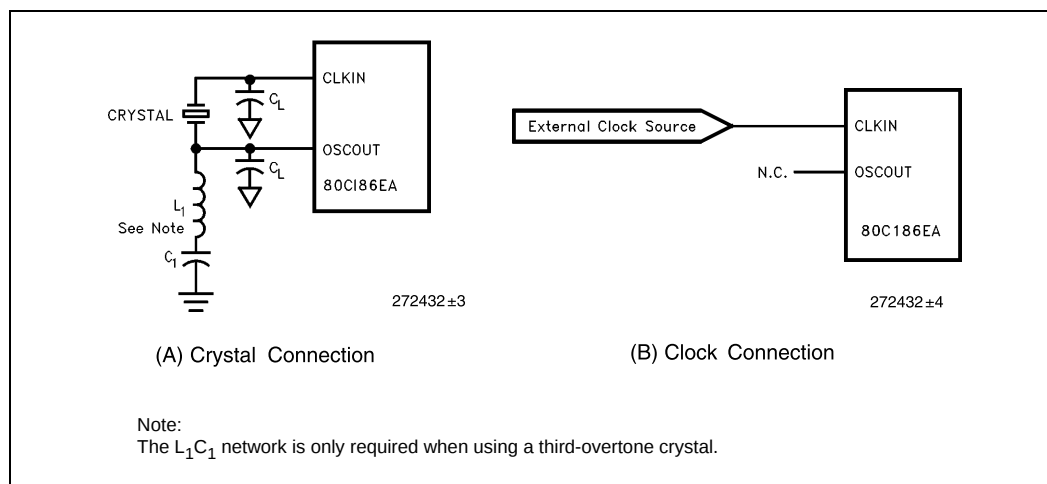
Figure 2. Clock Configurations
