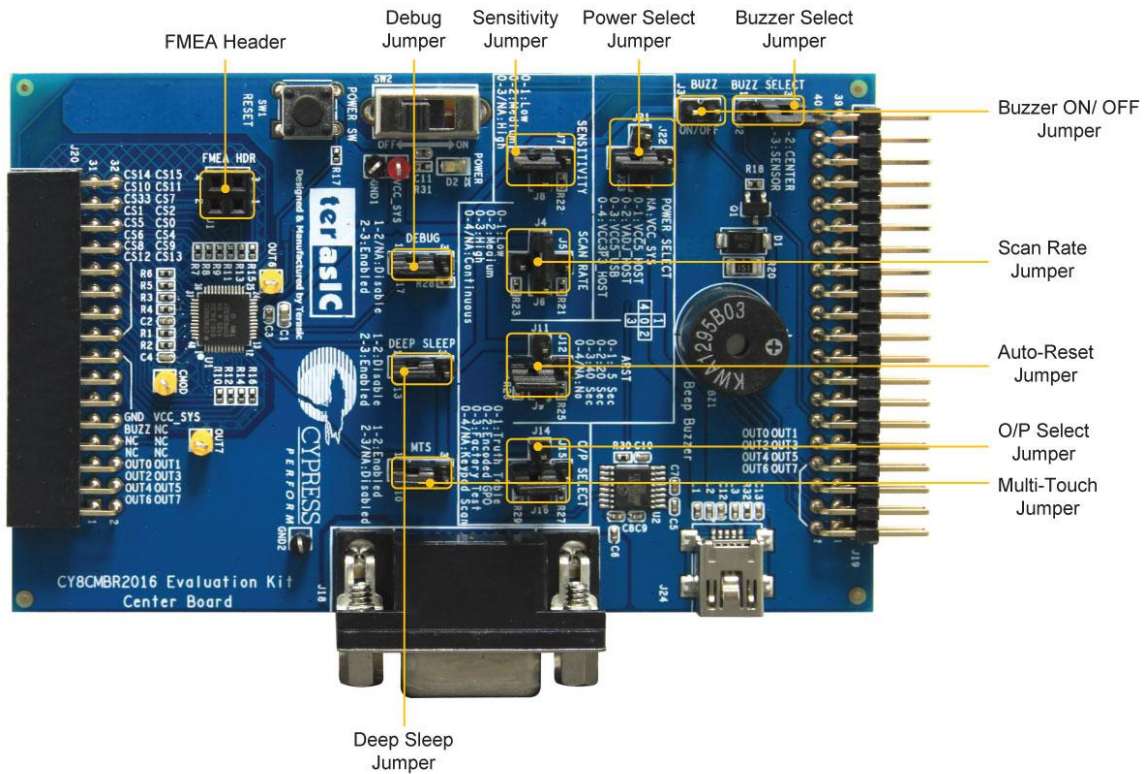
Figure 2-3 Jumper locations
