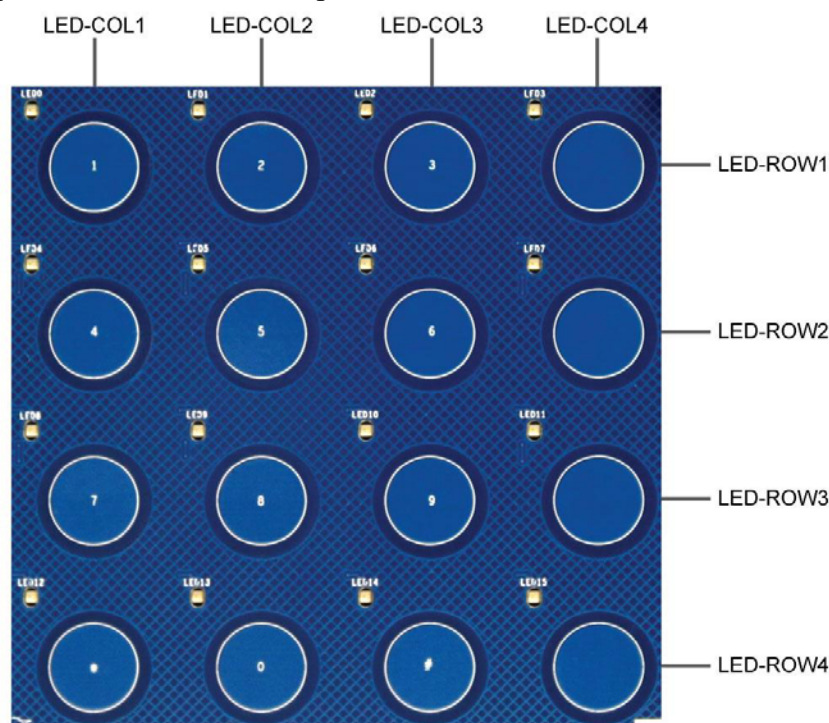
Figure 3-1 LED Arrangement
