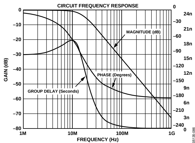
Figure 87. Filter Plot for Output Filter for SD, 16× Oversampling
