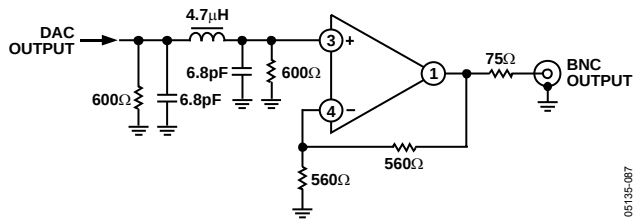
Figure 85. Example of Output Filter for PS, 8× Oversampling
