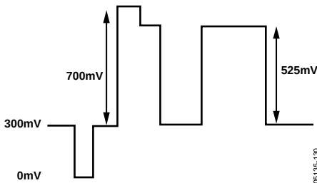
Figure 129. SD RGB Output Levels—RGB Sync Enabled
