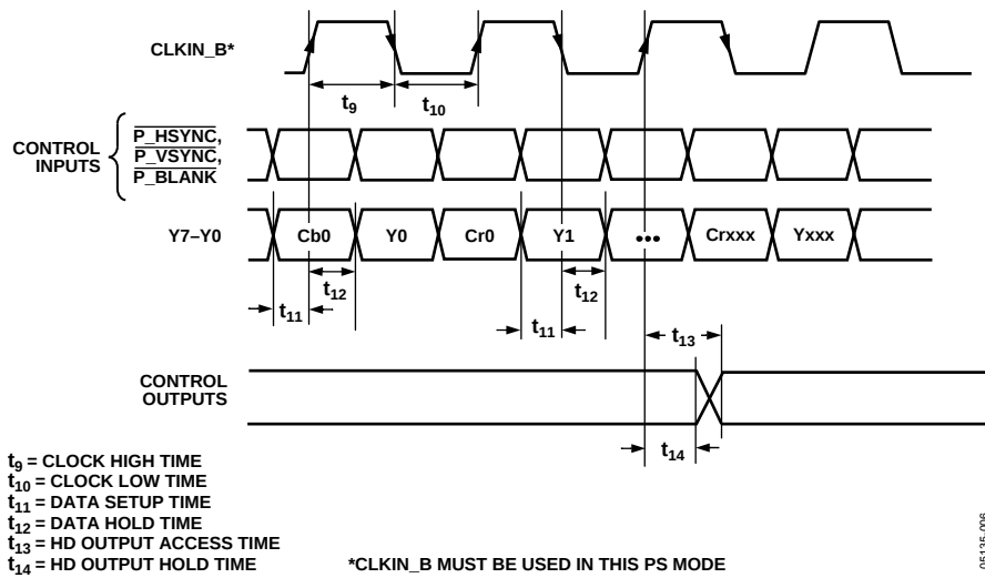
Figure 6. PS 4:2:2 8-Bit Interleaved at 27 MHz HSYNC/VSYNC Input Mode (Input Mode 100)
