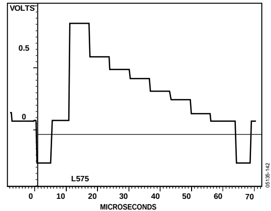
Figure 140. PAL Chroma
