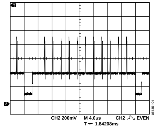
Figure 103. 625p Hatch Pattern
