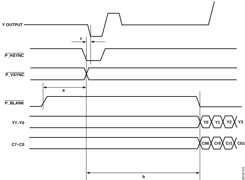
Figure 14. 16-Bit, SD-Only Pixel Input Mode (Input Mode 000)
