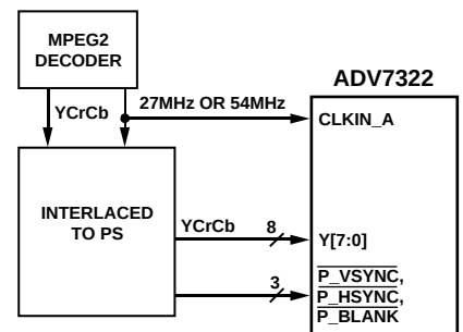
Figure 56. 8-Bit PS at 27 MHz or 54 MHz
