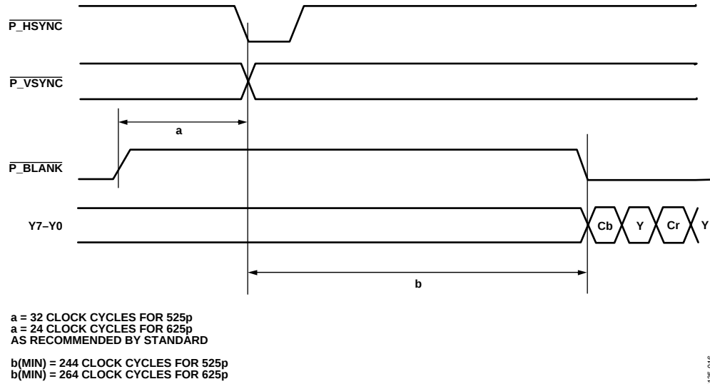
Figure 16. PS 4:2:2 8-Bit Interleaved Input Timing Diagram
