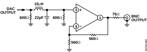
Figure 84. Example of Output Filter for SD, 16× Oversampling
