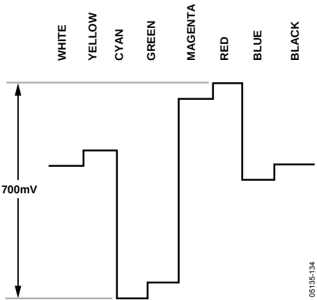
Figure 133. Pr Levels (PAL)
