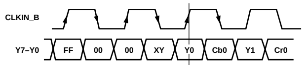
Figure 54. Input Sequence in PS Bit-Interleaved Mode (EAV/SAV)
