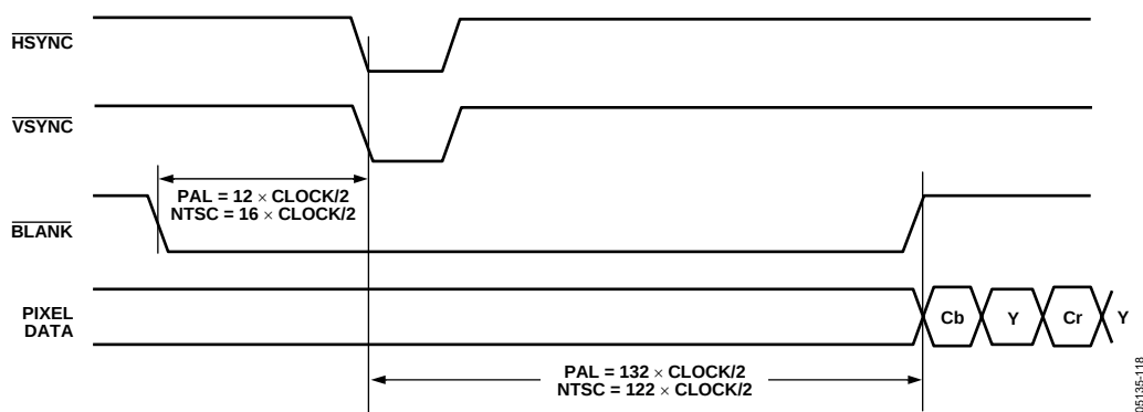
Figure 117. SD Timing Mode 2 Even-to-Odd Field Transition Master/Slave
