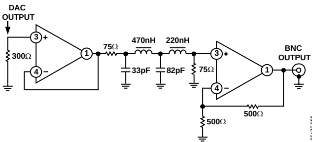
Figure 86. Example of Output Filter for HDTV, 2× Oversampling
