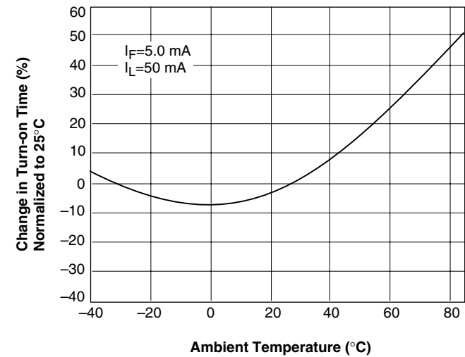
Figure 14. Turn-on Time vs. Temperature
