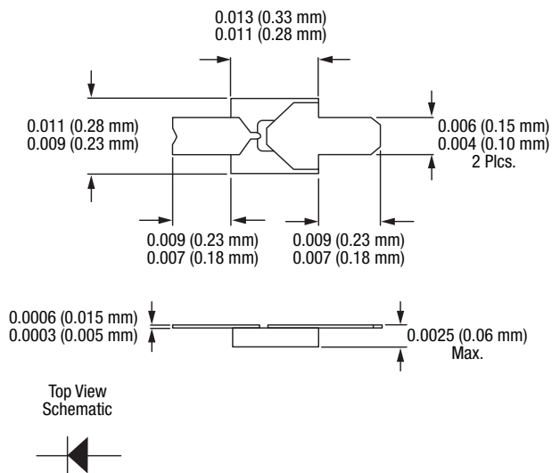
Figure 10. 491-006 Package Dimensions
