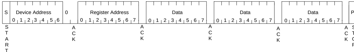
Figure 4-6: I 2 C Bus 3-byte Data Write
