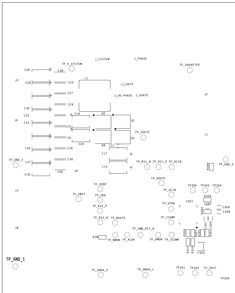
FIGURE 8. BOTTOM SILKSCREEN
