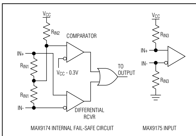
Figure 1. Input Structure
