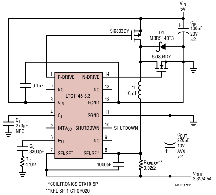
Figure 14. High Efficiency 5V to 3.3V/4.5A Converter
