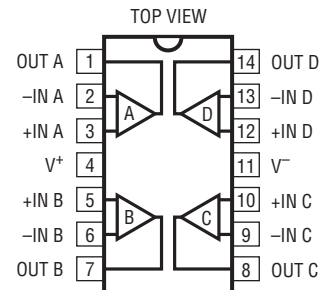
N PACKAGE 14-LEAD PDIP
