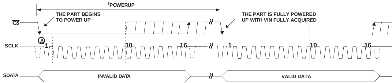
Figure 7. Exiting Power Down Mode
