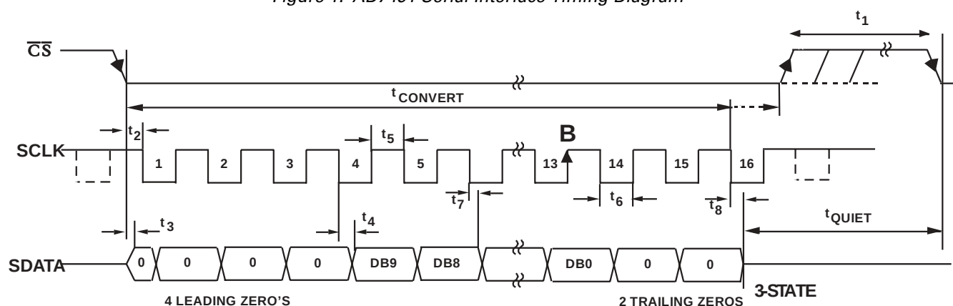
Figure 2. AD7441 Serial Interface Timing Diagram
