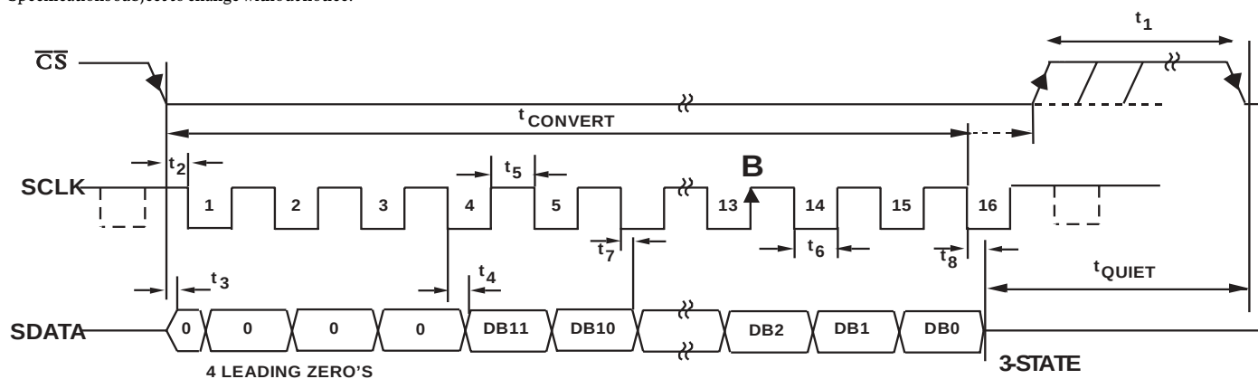
Figure 1. AD7451 Serial Interface Timing Diagram
