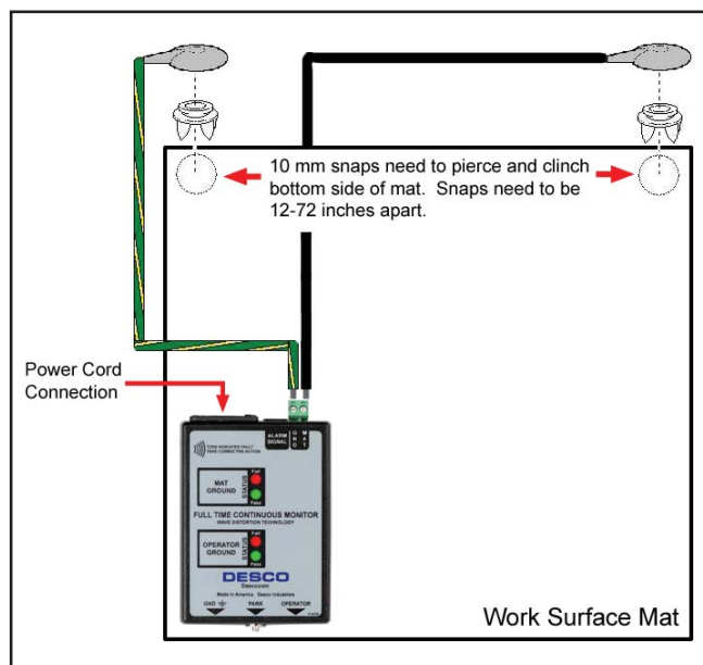
Figure 3. Installation of the Full Time Continuous Monitor
