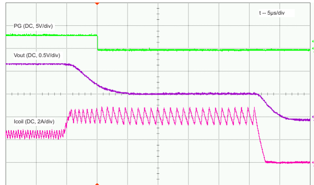
Figure 9-19. Output Short-Circuit Protection, Load = 0.47 Ω, HICCUP Zoom In
