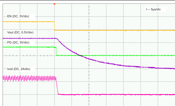
Figure 9-13. Shutdown, Load = 0.47 \Omega
