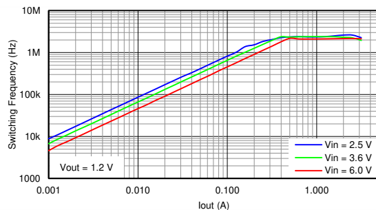
Figure 7-1. Switching Frequency
