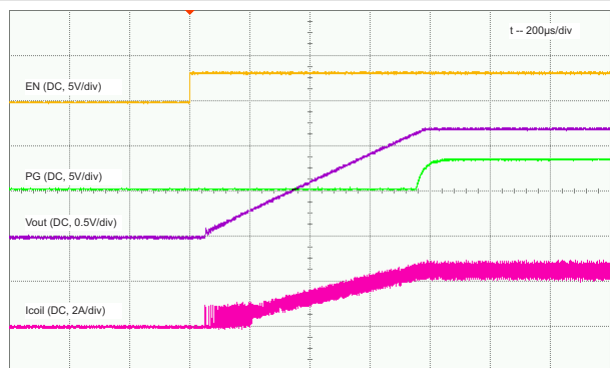
Figure 9-11. Start-Up, Load = 0.47 \Omega
