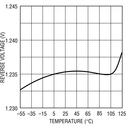
Temperature Drift
