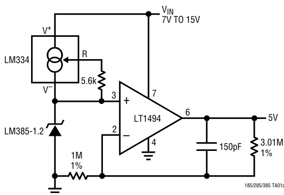
Micropower 5V Reference
