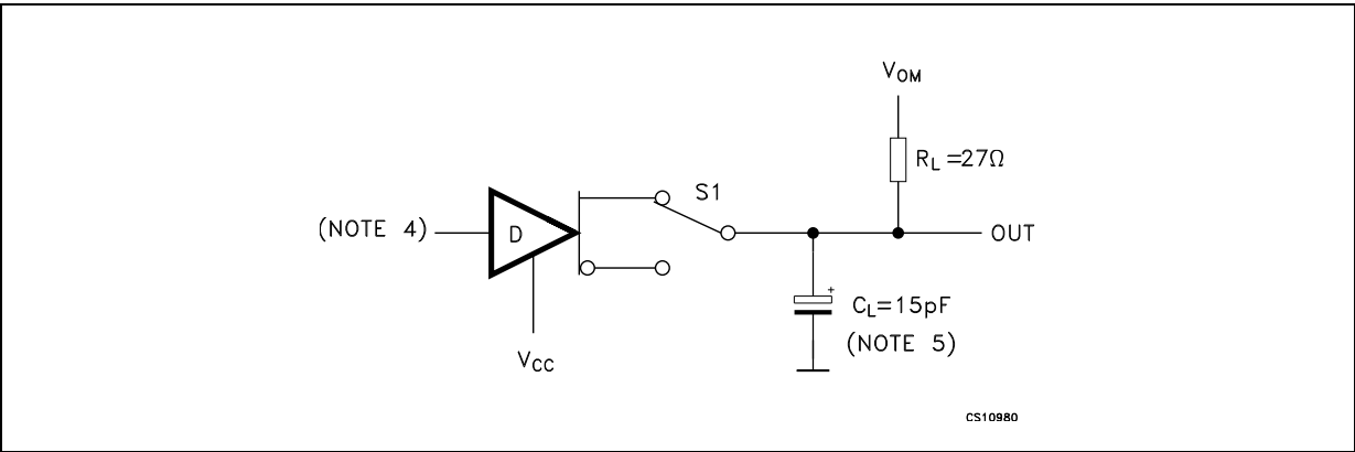
Figure 10. Drive propagation time test circuit
