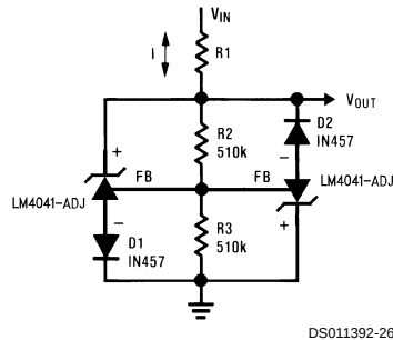
FIGURE 7. Bidirectional Clamp ±2.4V
