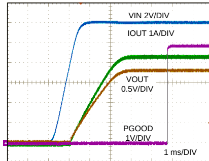
Figure 32. Startup
