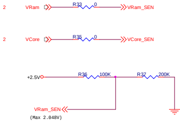
Voltage sensing circuit
