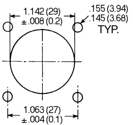
Mounting Dimensions
