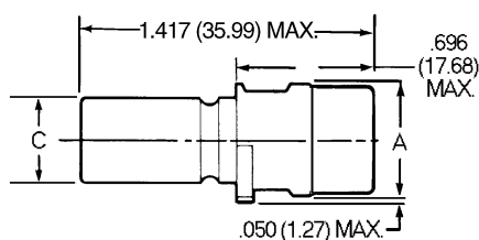
Plug
