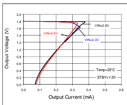
Fig 9. OCP Threshold
