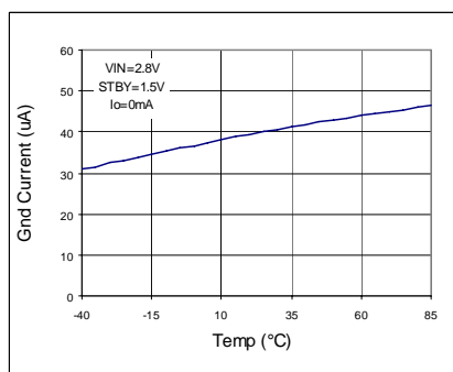
Fig 12. IGND - Temp
