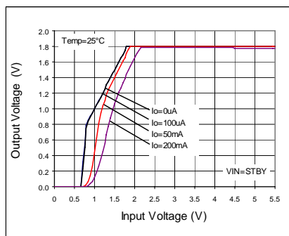
Fig 3. Output Voltage
