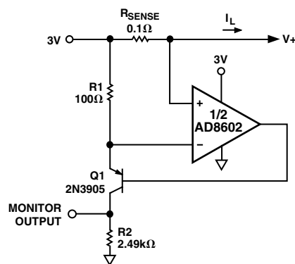
Figure 5. A High-Side Current Monitor
