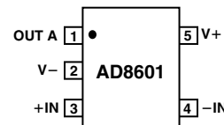
5-Lead SOT-23 (RT Suffix)
