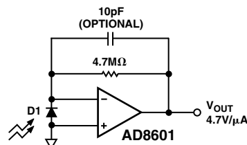
Figure 3. Amplifier Photodiode Circuit
