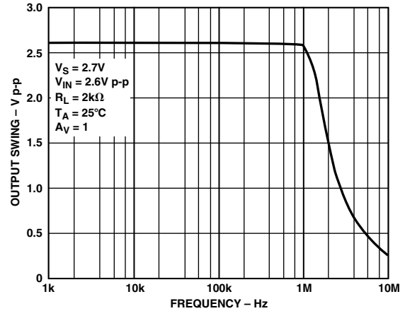
TPC 22. Closed-Loop Output Voltage Swing vs. Frequency
