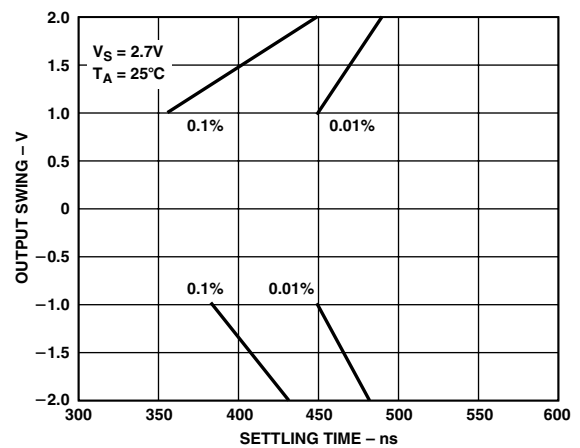
TPC 48. Output Swing vs. Settling Time
