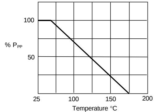
Figure 4 - Derating Curve
