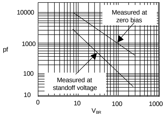
Figure 3 - Typical Capacitance
