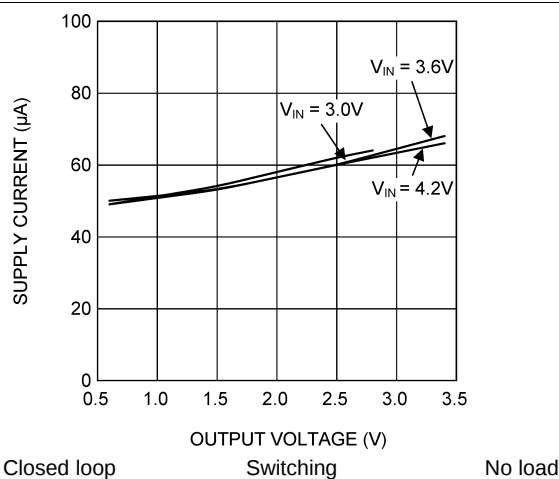
Figure 3. Eco-mode Supply Current vs Output Voltage
