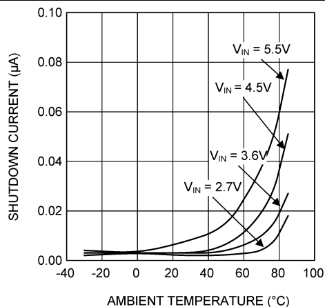
Figure 1. Shutdown Current vs Temperature
