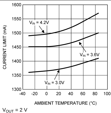
Figure 11. Closed-loop Current Limit vs Temperature
