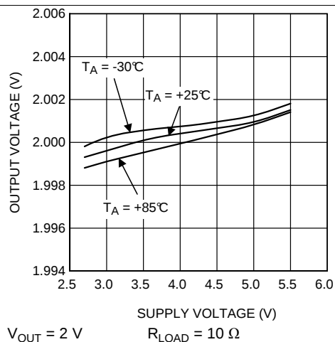
Figure 5. Output Voltage vs Supply Voltage
