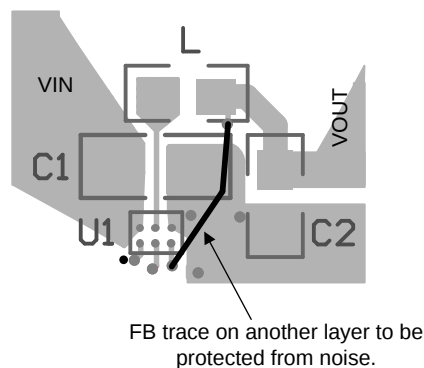
Figure 32. Feedback Trace
