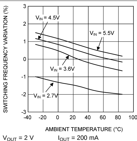
Figure 4. Switching Frequency vs Temperature
