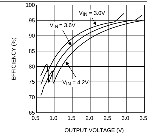
Figure 14. Efficiency vs Output Voltage
