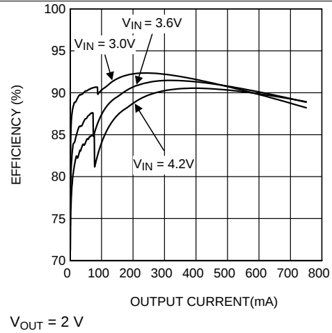
Figure 12. Efficiency vs Output Current
