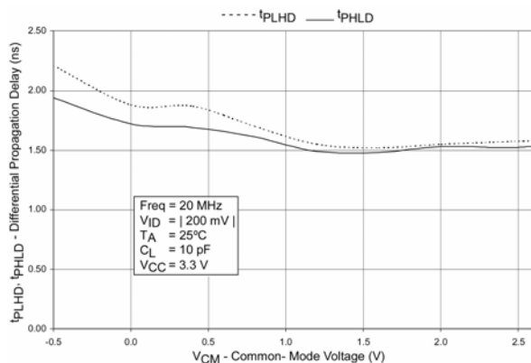
Figure 14. Differential Propagation Delay vs. Common-Mode Voltage
