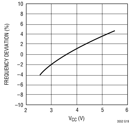
Oscillator Frequency Error vs V_{CC}
