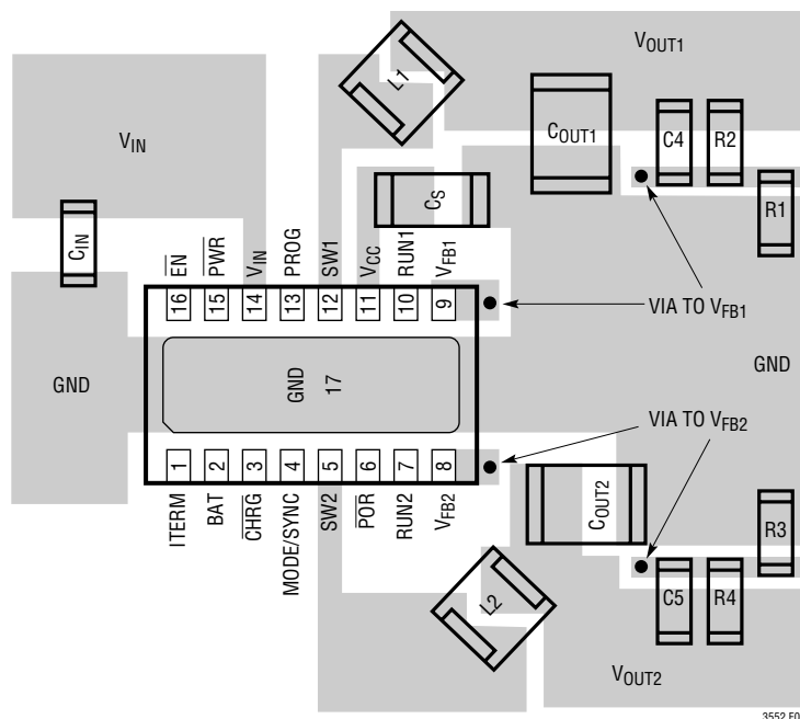
Figure 6. Suggested Layout
