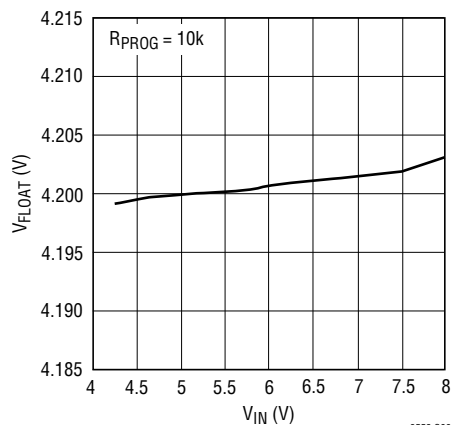
Regulated Output (Float) Voltage vs V_{IN}
