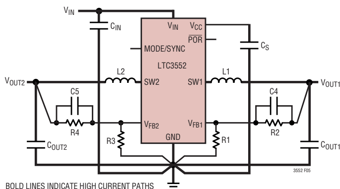
Figure 5. Layout Diagram
