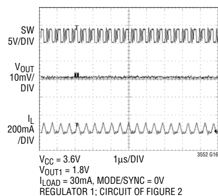
Pulse-Skipping Mode
