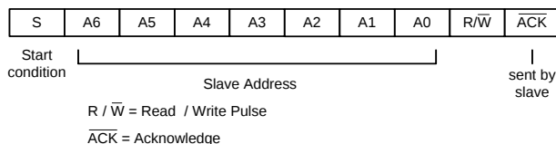
Figure 26. Slave Address Transfer Format
