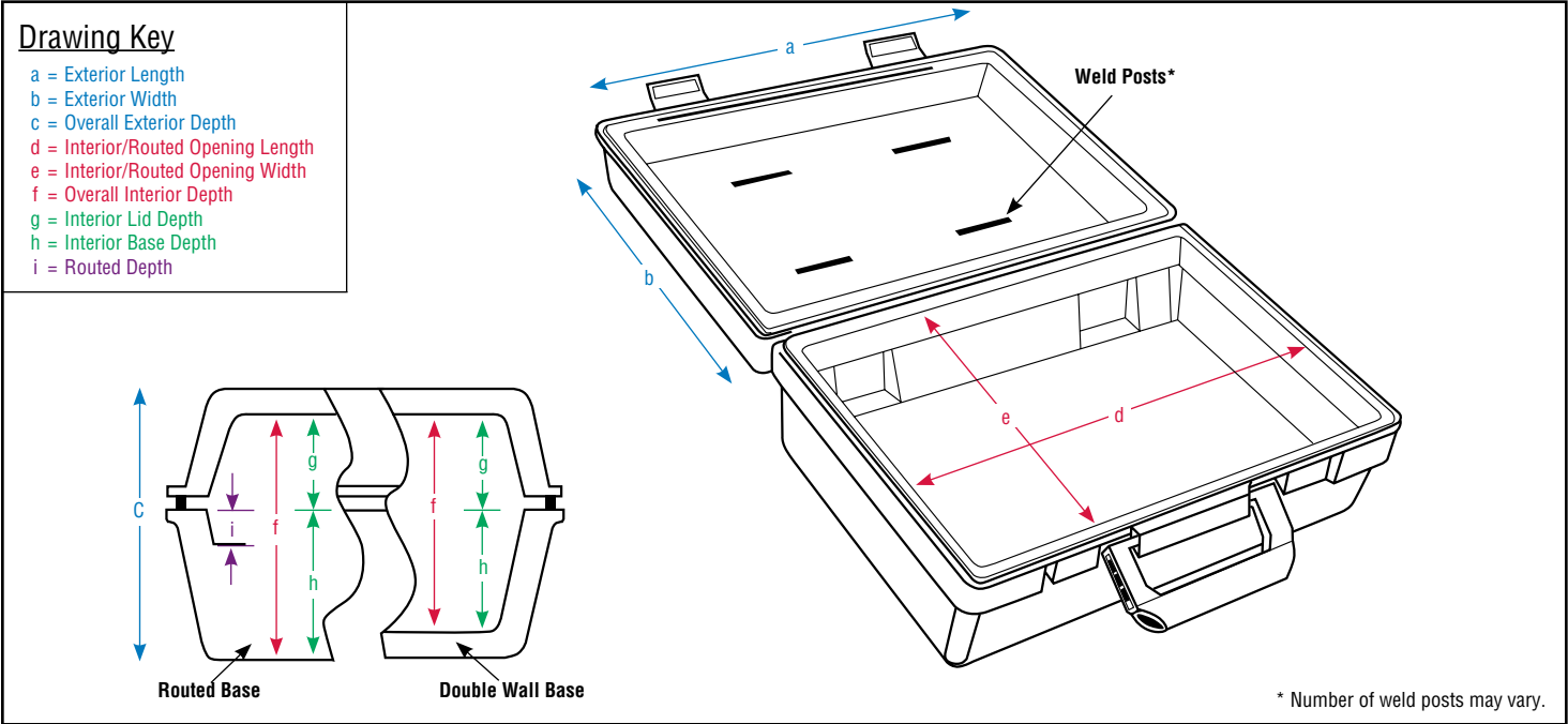
“R” Series Integral Hinge
