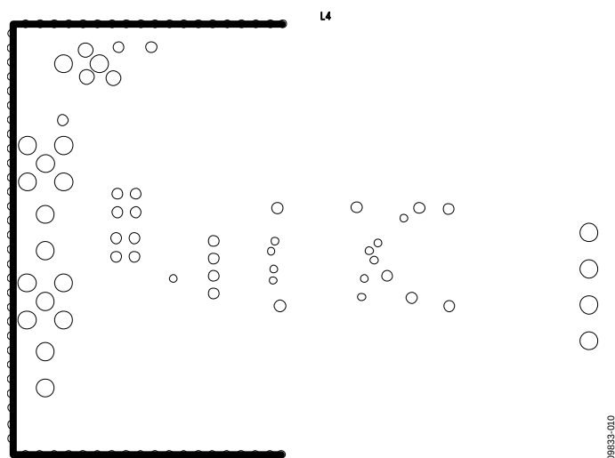
Figure 9. ADM3053 Evaluation Board Layer 4
