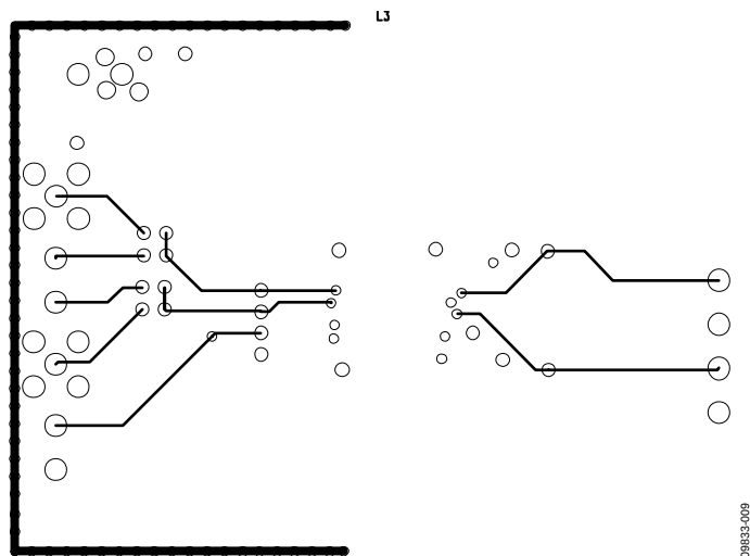
Figure 8. ADM3053 Evaluation Board Layer 3
