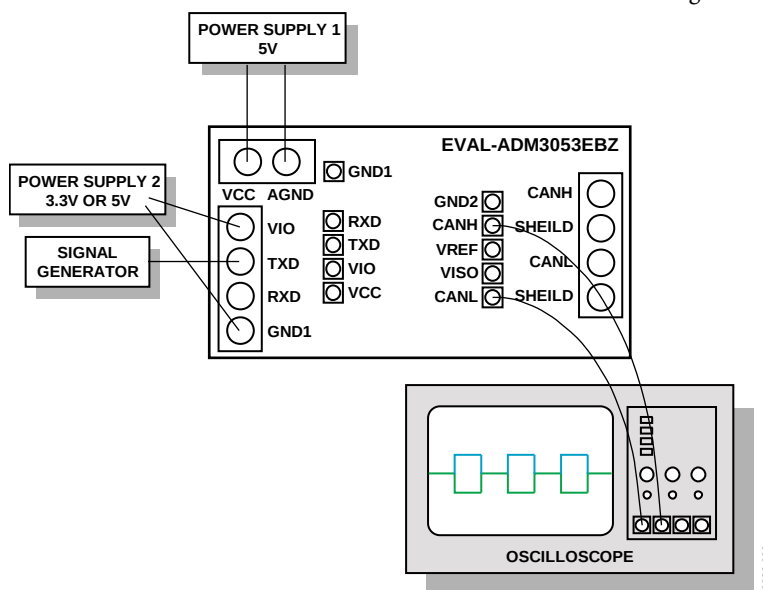
Figure 2. Basic Isolated CAN Transceiver Evaluation Board Operation
