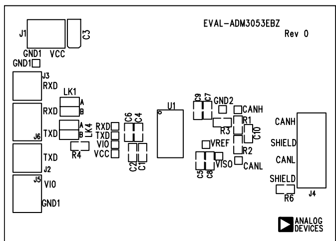
Figure 5. ADM3053 Evaluation Board Silkscreen
