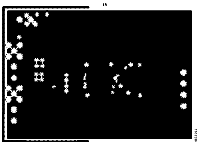
Figure 10. ADM3053 Evaluation Board Layer 5
