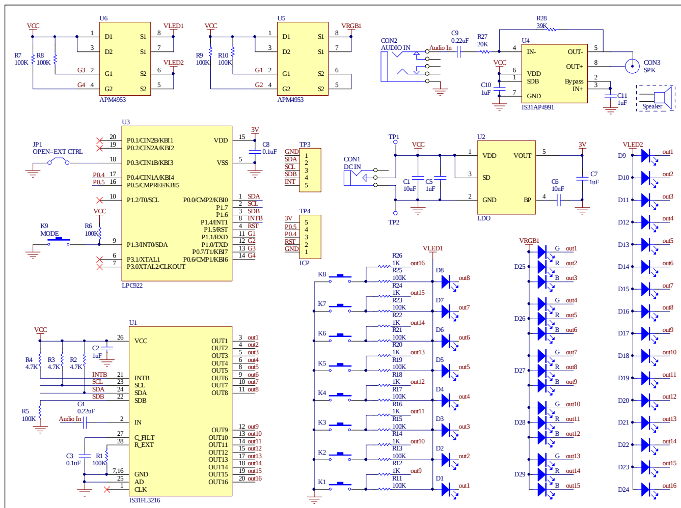
Figure 2: IS31FL3216 Application Schematic
